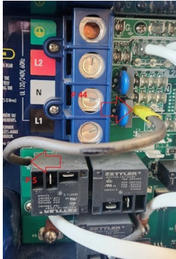
FIGURE 1: 120 VOLT CONFIGURATION
